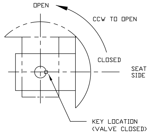
PLUG POSITIONS VIEWED FROM TOP
